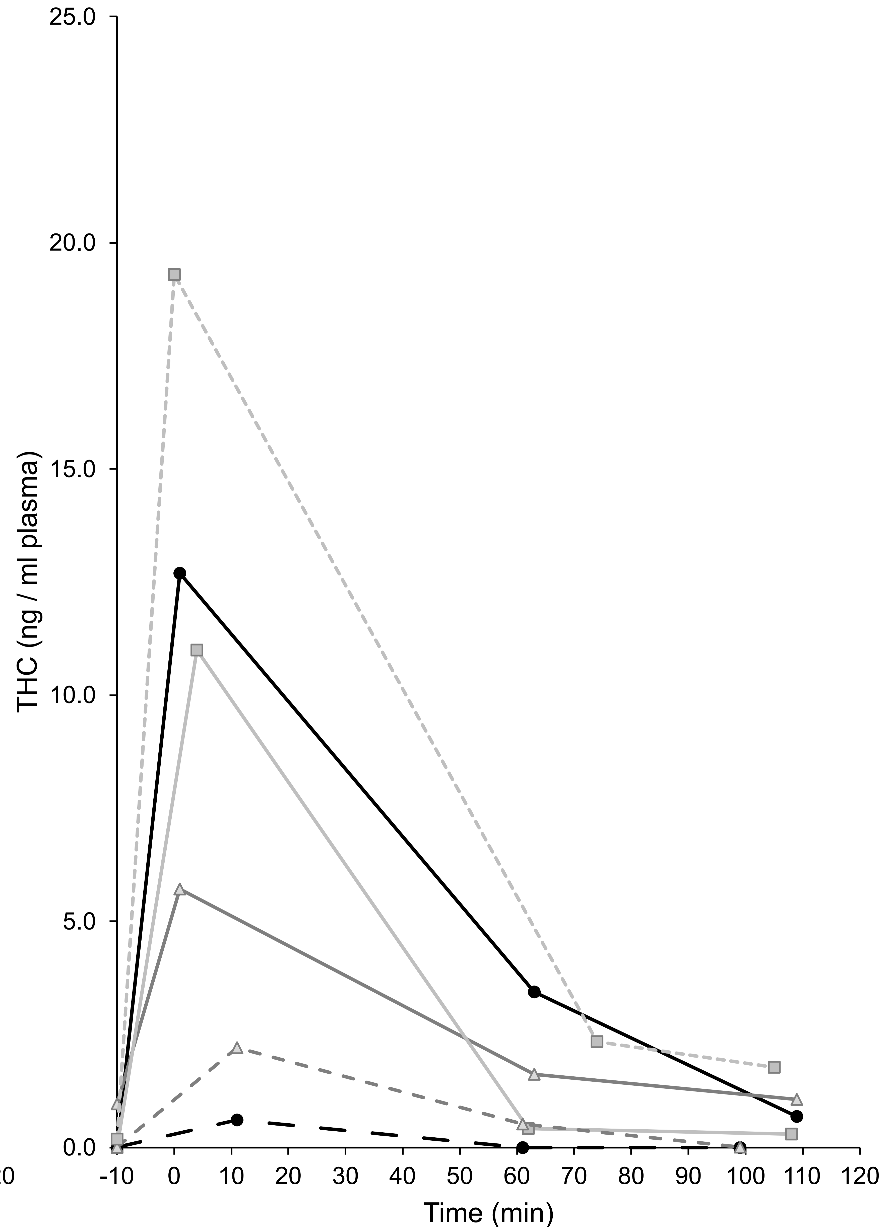
THC in plasma at different timepoints
