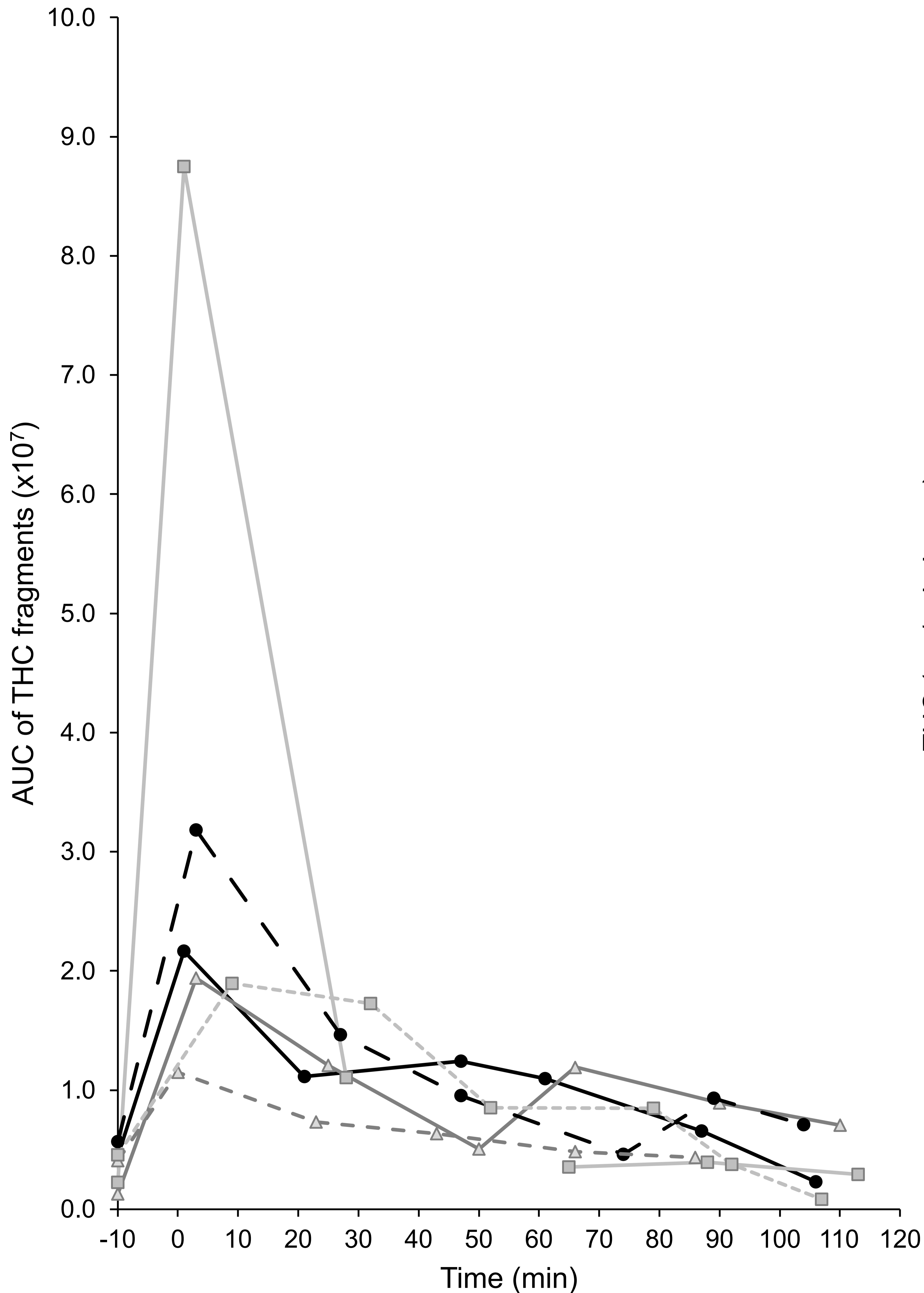
THC in breath at different timepoints
